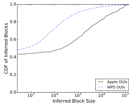
Figure 4: CDFs of Inferred Block Sizes for WPS-Using Manufacturers and Apple
