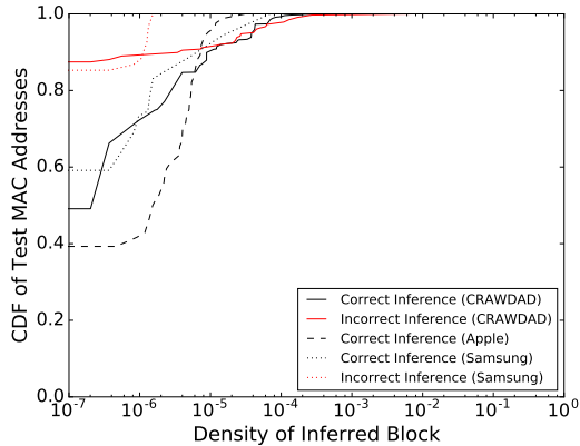
Figure 10: Relationship between observation density and inference ability
